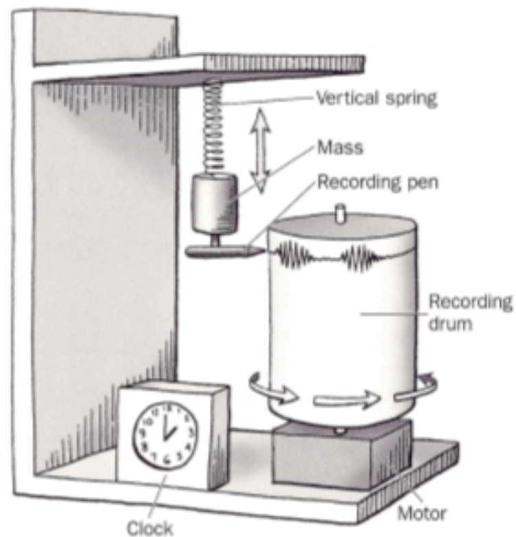
Figure 12.2 A vertical seismograph contains a mass suspended from a spring. The mass and pen tend to remain still, while the rest of the instrument moves up and down. As a result, vertical ground motions can be recorded.
