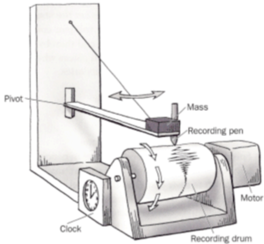
Figure 12.1 Horizontal seismograph
