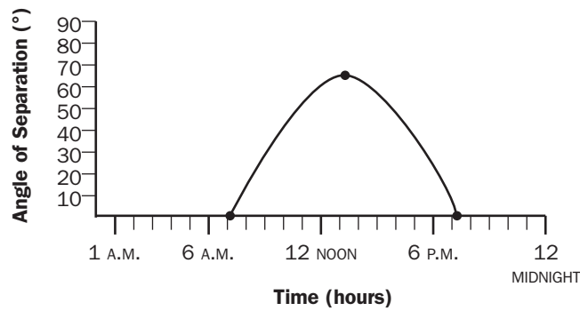
Figure 4.6 Sample drawing of the ecliptic for Quito, Ecuador, on June 21
